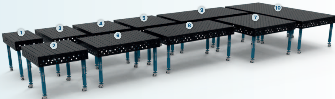
DIMENSIONS OF EXPERT , PRO , PLUS and ECO TABLES [mm].
